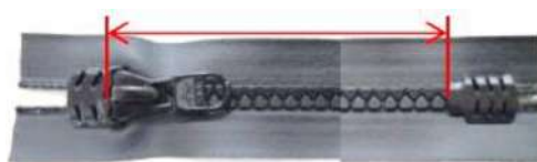
Zipper length is measured from the top of slider to the end of element/top of bottom stop for VISLON® zippers.
