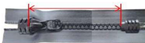
Zipper length is measured from the top of slider to the end of element/top of bottom stop for VISLON® item.
